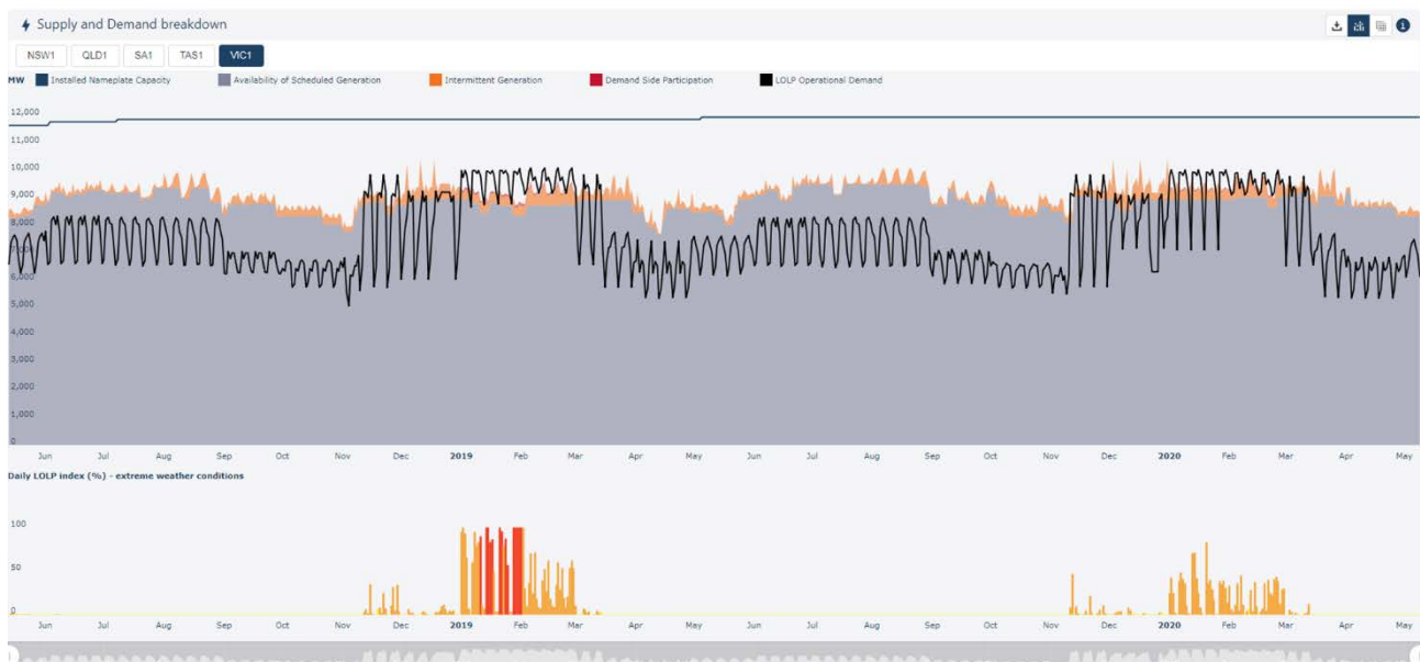
Figure 13: Supply demand breakdown & maintenance period overview from LOLP Run (User to select Region and Year)
