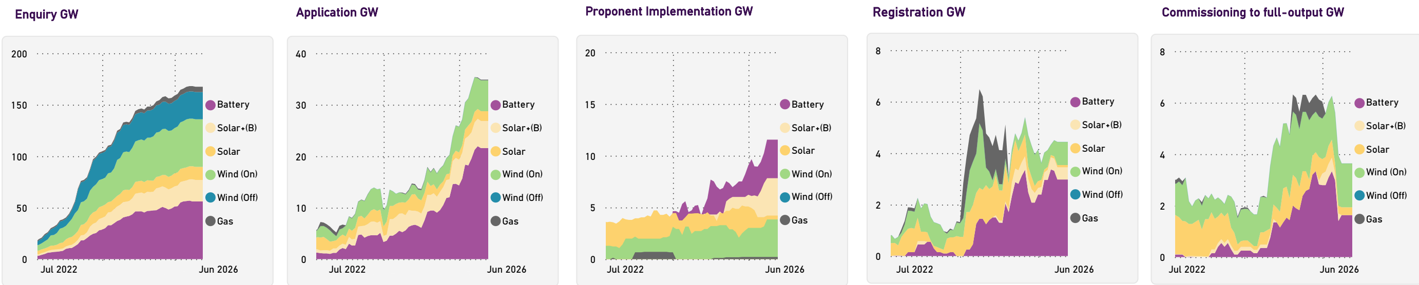
Fig. 6 GW Volume Trend Analysis by Major Technologies
