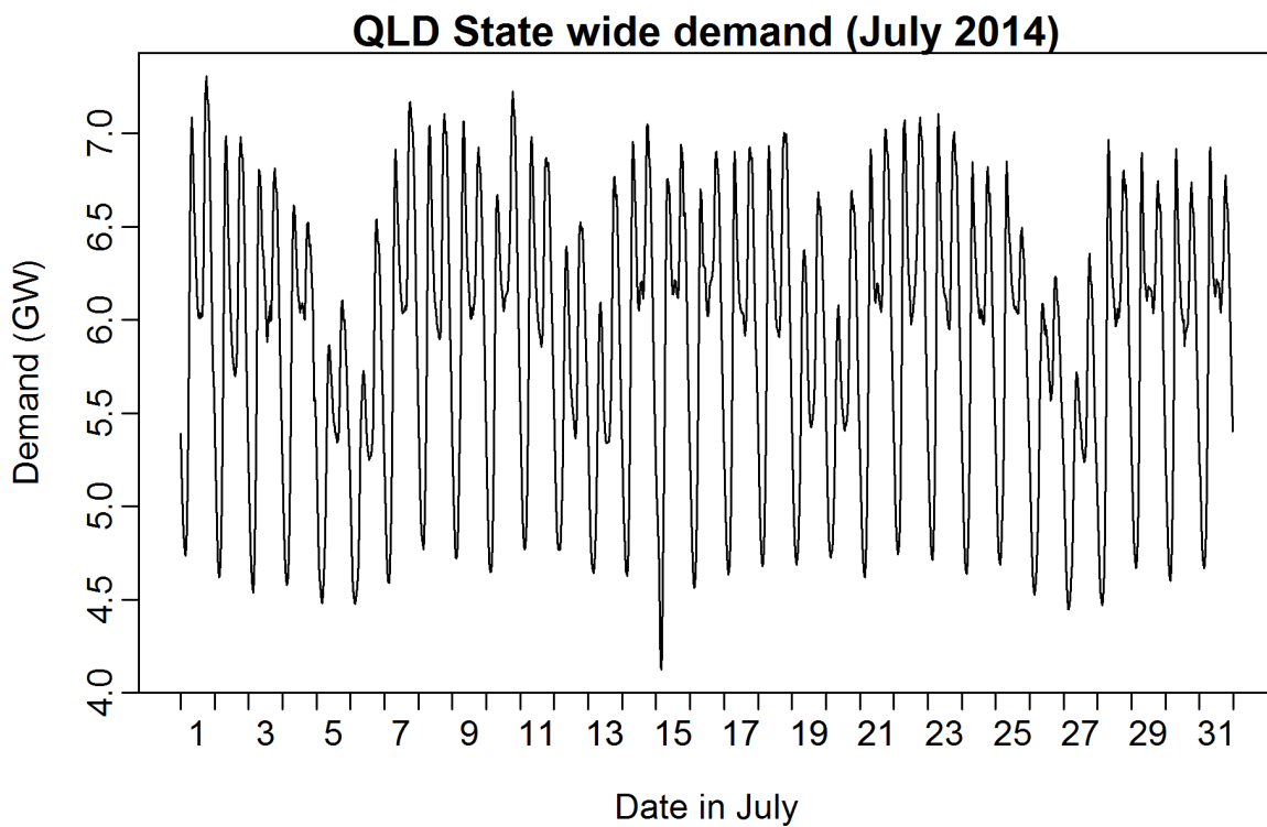
Figure 29: Half-hourly demand data for Queensland, July 2014.
