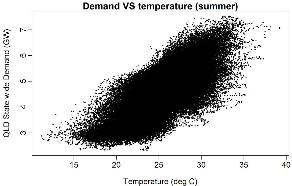
Figure 7: Half-hourly QLD electricity demand (excluding major industrial demand) plotted against average temperature (degrees Celsius).
