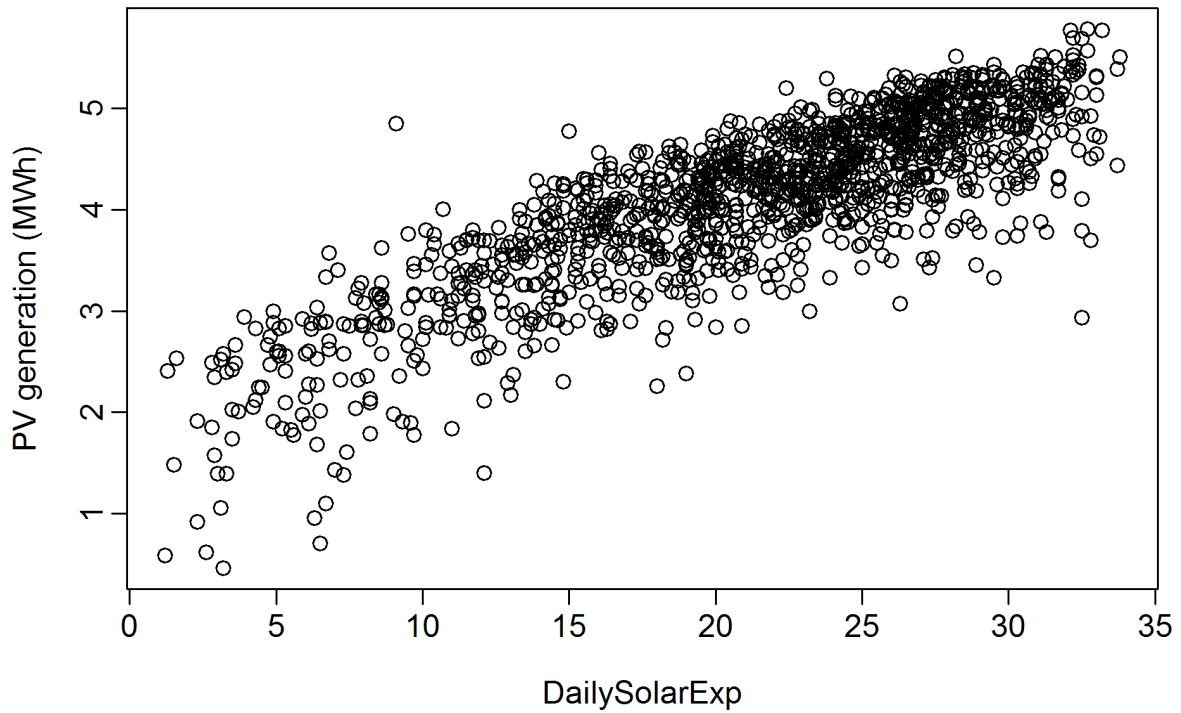
Figure 14: Daily solar PV generation plotted against daily solar exposure data in QLD from 2003 to 2011. Only data from October–March are shown.
