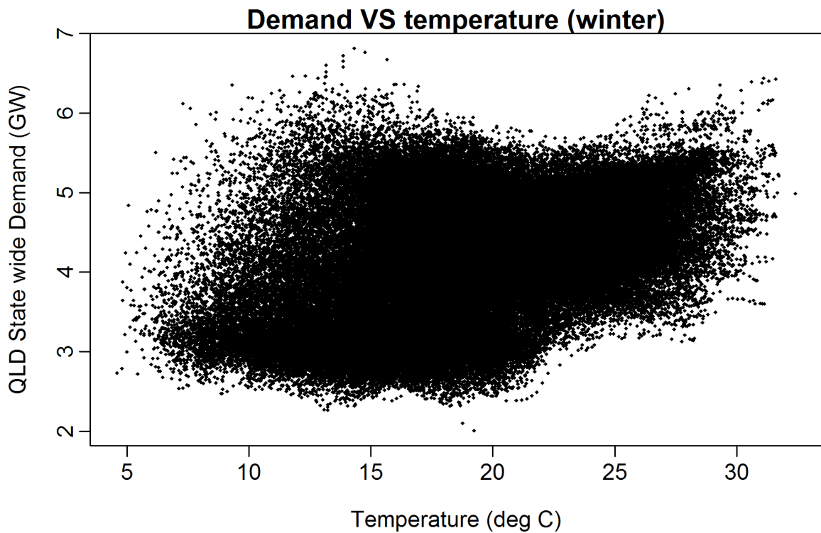
Figure 33: Half-hourly QLD electricity demand (excluding major industrial demand) plotted against average temperature (degrees Celsius).
