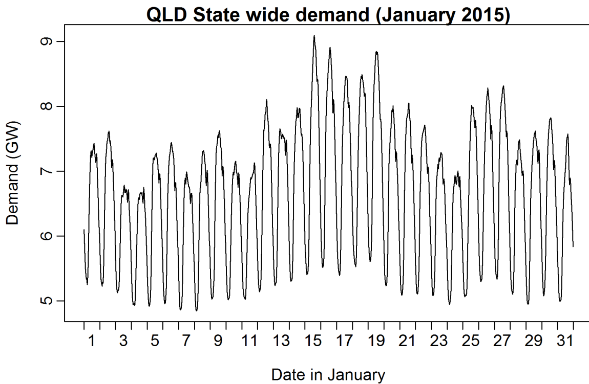
Figure 3: Half-hourly demand data for Queensland, January 2015.
