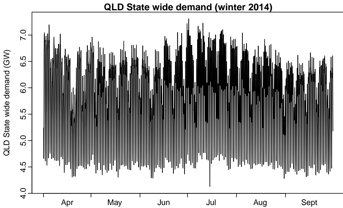
Figure 28: Half-hourly demand data for Queensland for last winter.
