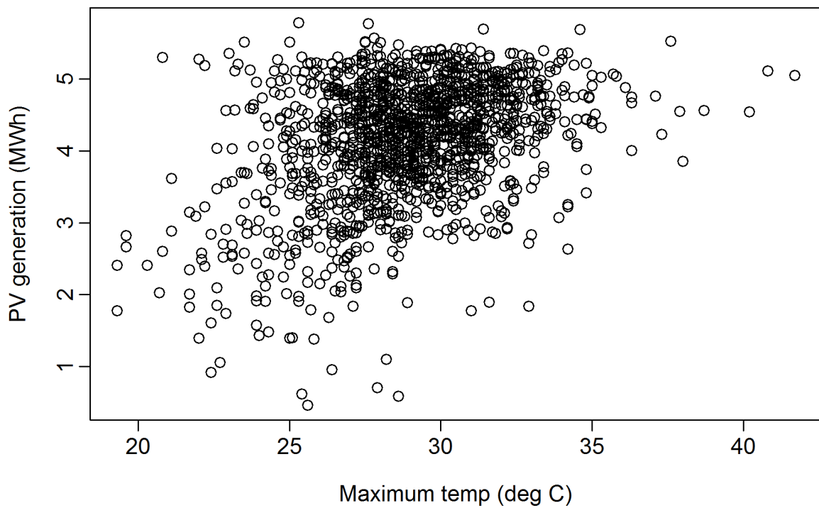
Figure 15: Daily solar PV generation plotted against daily maximum temperature in QLD from 2003 to 2011. Only data from October–March are shown.
