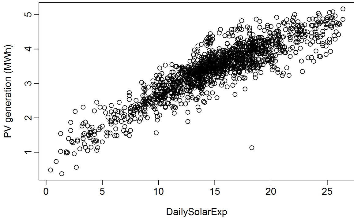
Figure 39: Daily solar PV generation plotted against daily solar exposure data in QLD from 2003 to 2011. Only data from April–September are shown.
