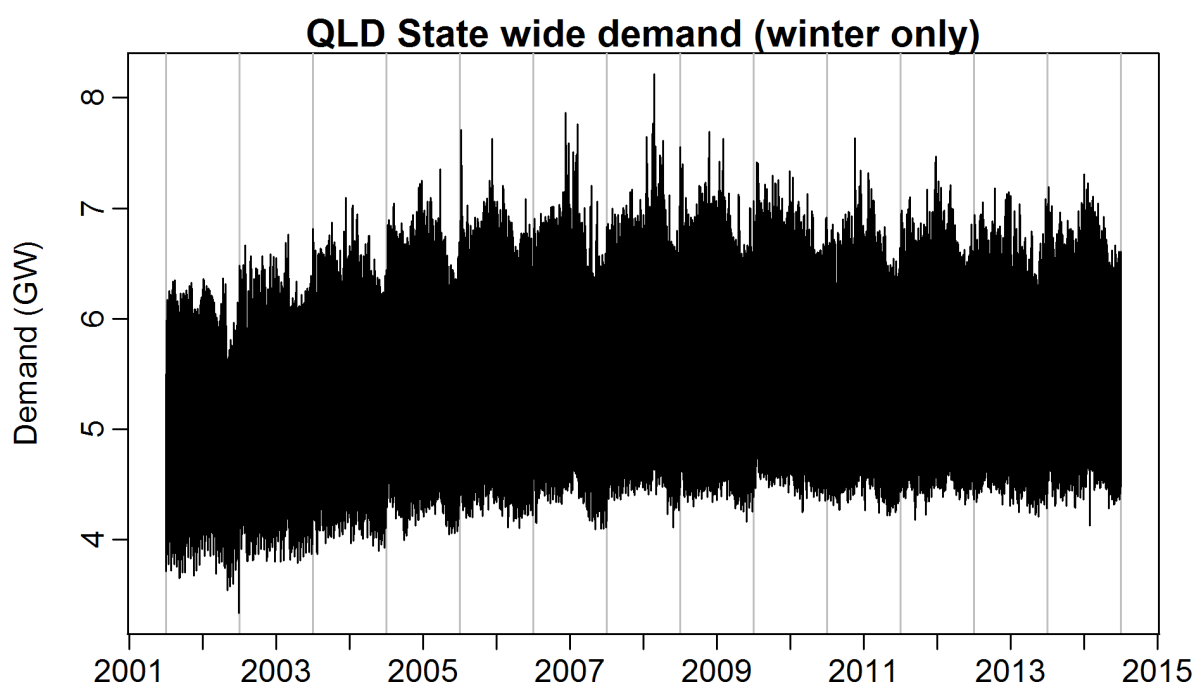
Figure 27: Half-hourly demand data for Queensland from 2002 to 2015. Only data from April–September are shown.
