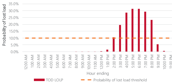
Figure 5 Time of day probability of lost load assessment (all months)
