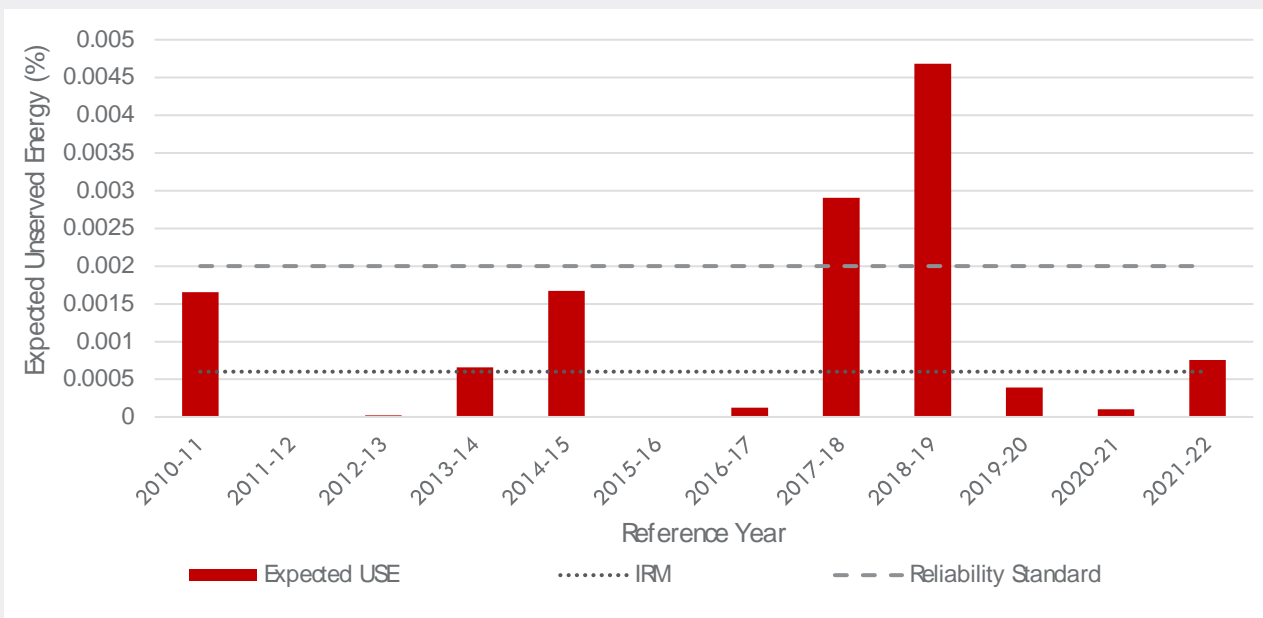
Figure 4 Unserved energy by Reference Year
