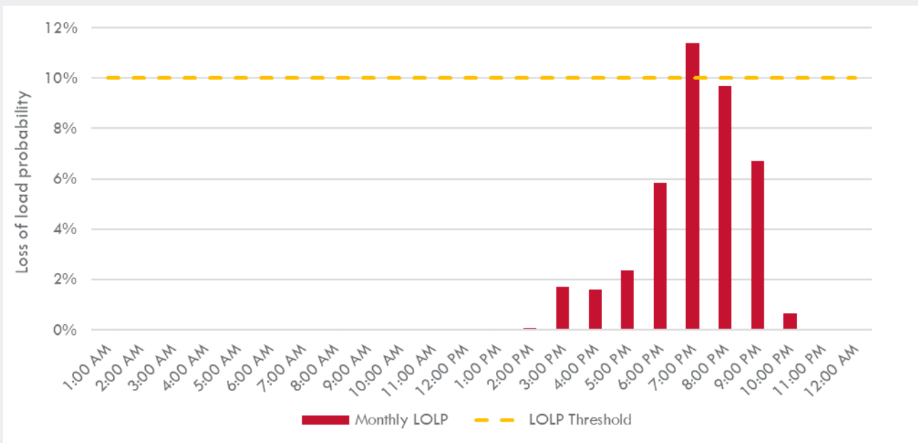
Figure 7 Time of day probability of lost load assessment (all identified months)
