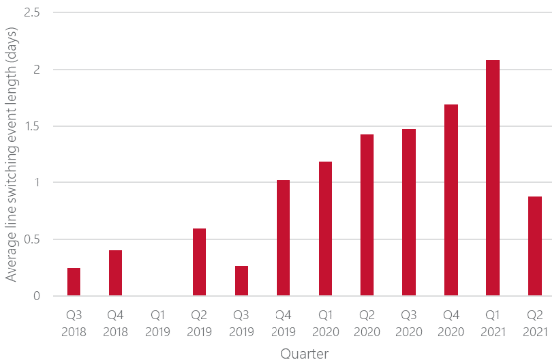
Figure 8 Average periods during which 500 kV lines are switched out to manage high voltage during low demand
