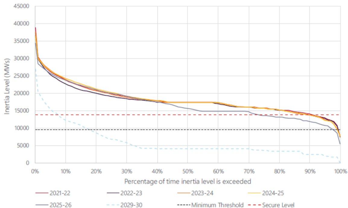
Figure 29 Projected inertia in Victoria
