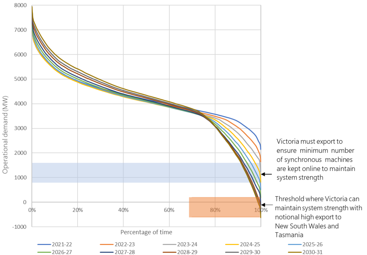
Figure 28 Operational demand projection duration curves by financial year
