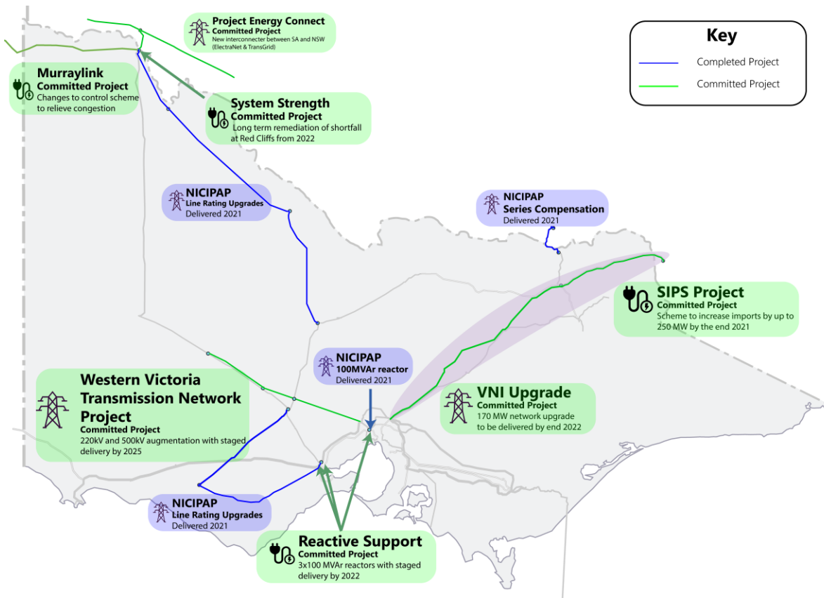
Figure 22 Transmission development plan – delivered and committed projects
