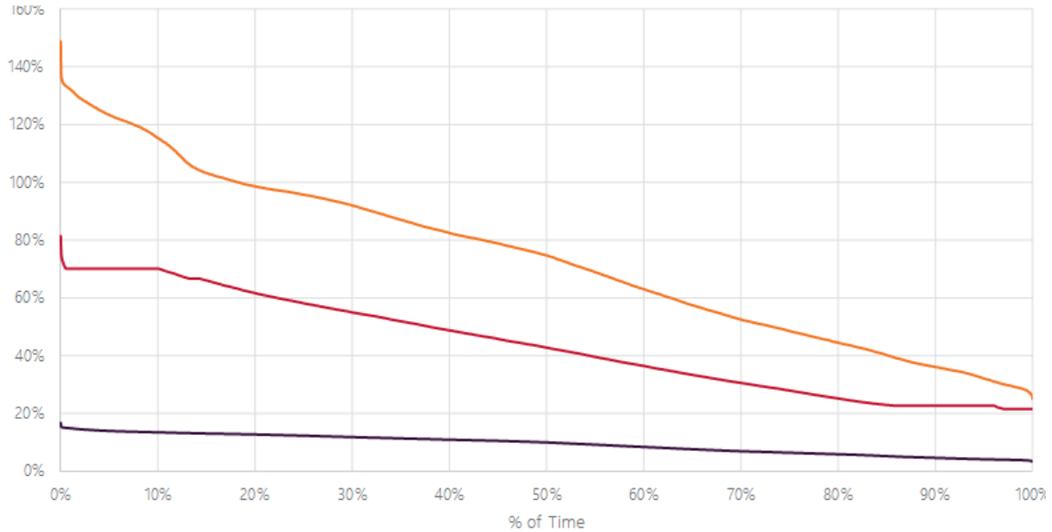
Figure 37 HWPS – YPS 220 kV line load (under contingency) duration curve
