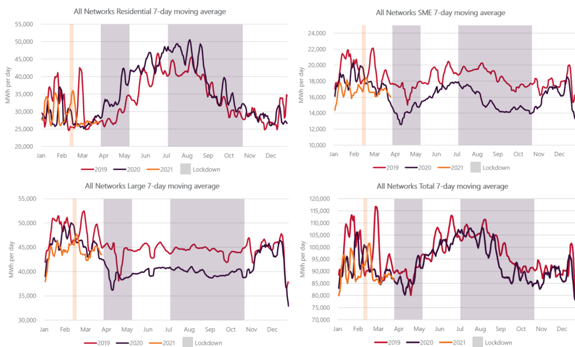
Figure 10 Seven-day moving average consumption (provided by AusNet Services)
