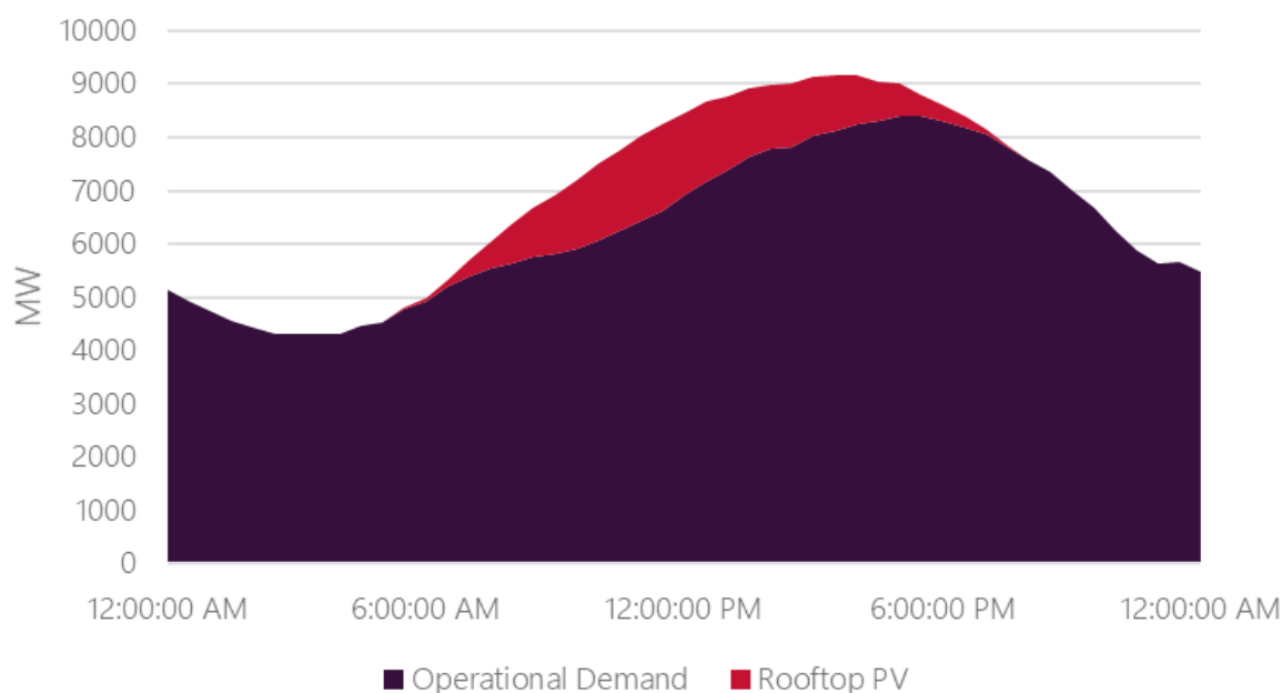
Figure 13 Victorian demand profile of maximum demand day (11 January 2021)
