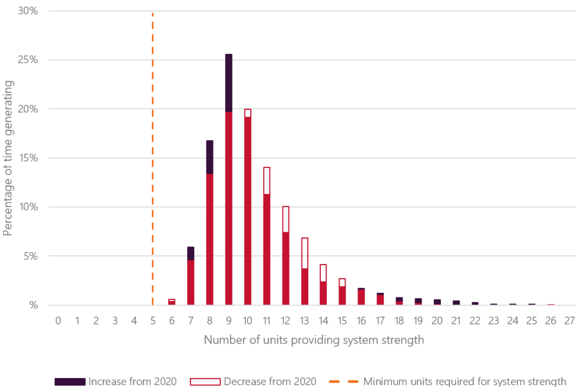
Figure 9 Available system strength units during 2019-20 (including Bogong and Murray 2)
