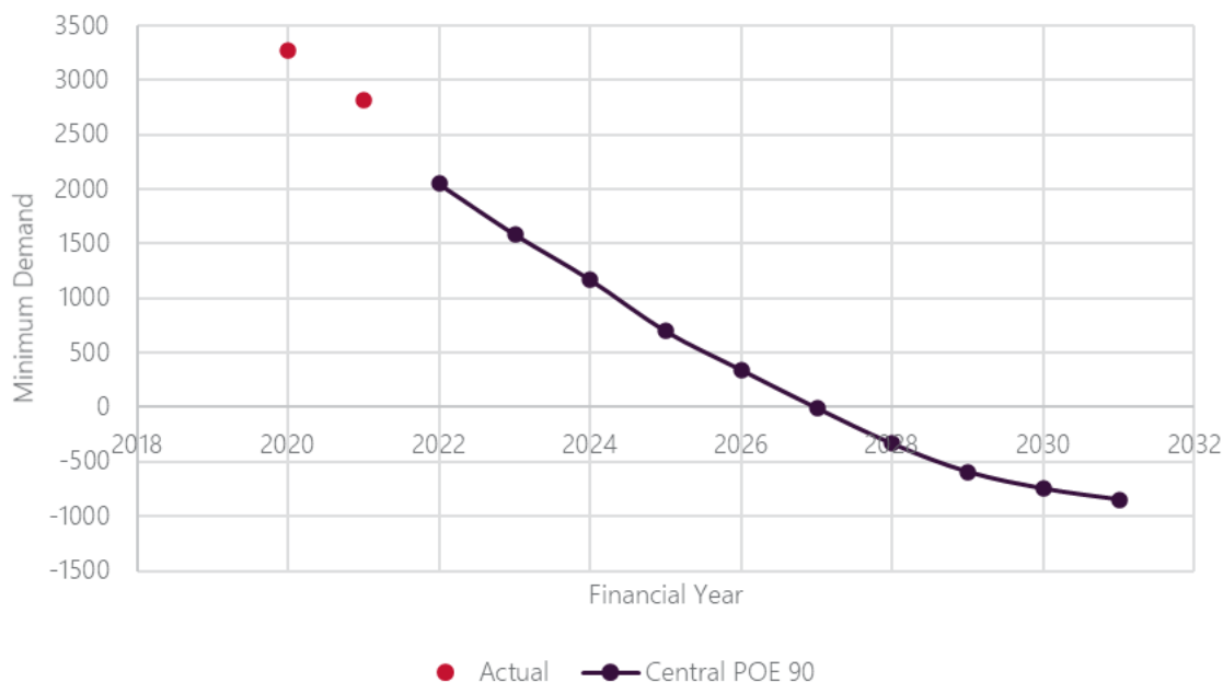
Figure 30 2021 ESOO forecast 90% POE shoulder minimum operational demand (sent-out) for Victoria (Central scenario)
