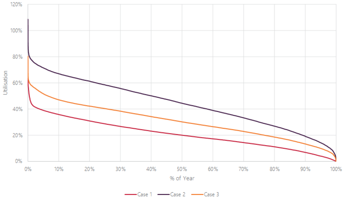
Figure 39 TSTS – TTS 220 kV line load (under contingency) duration curve
