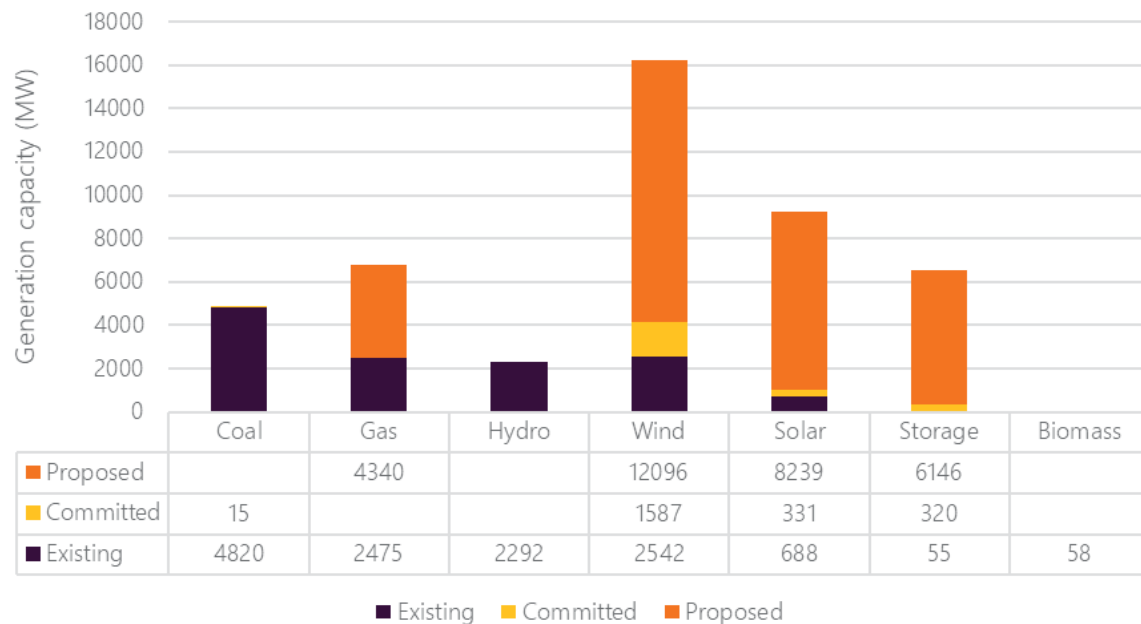
Figure 1 Current, committed, and proposed large-scale generation and storage in Victoria
