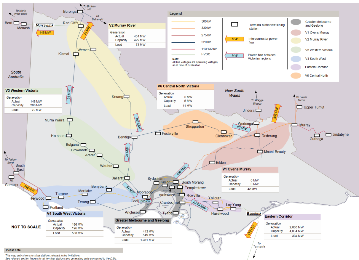
Figure 14 Minimum demand snapshot – generation, load, and interconnector flow
