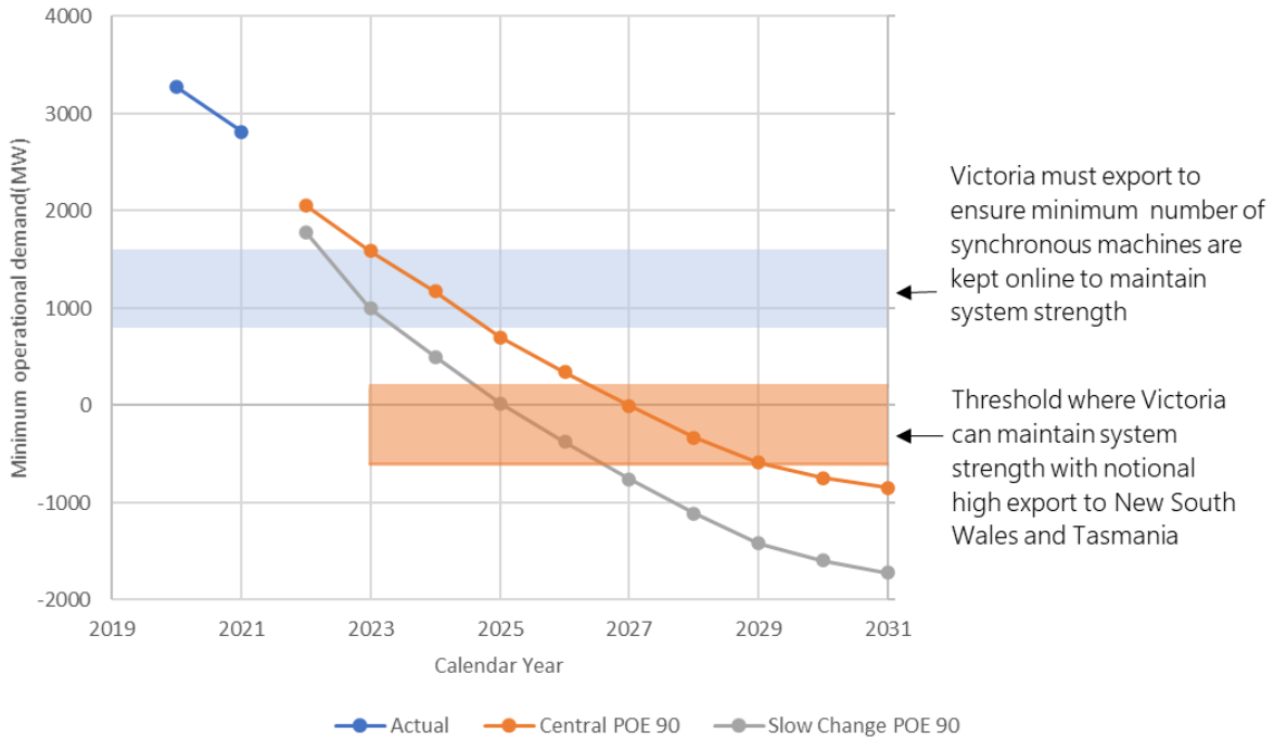
Figure 27 Minimum operational demand thresholds in Victoria
