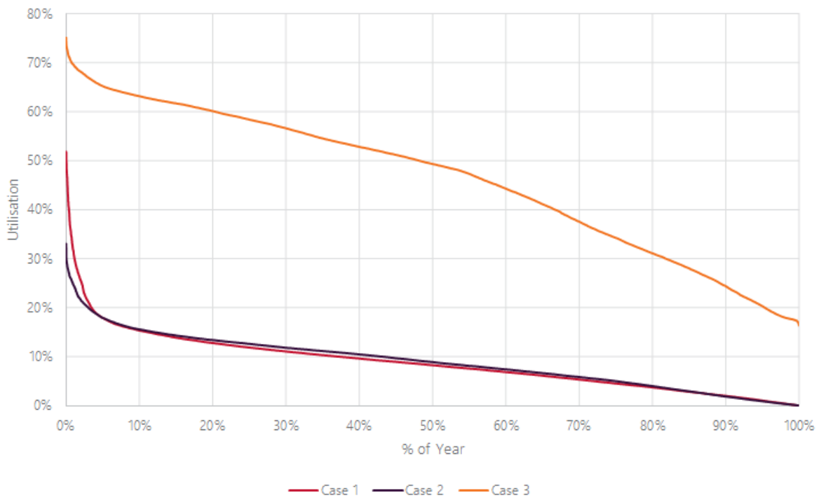
Figure 36 HWTS transformer load (under contingency) duration curve
