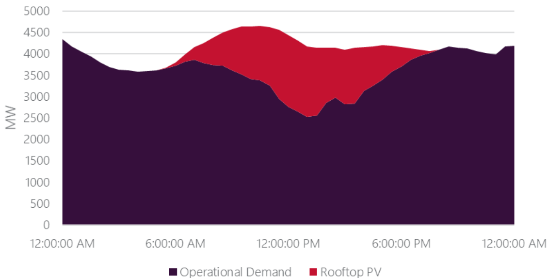
Figure 15 Victorian demand profile of minimum demand day (25 December 2020)
