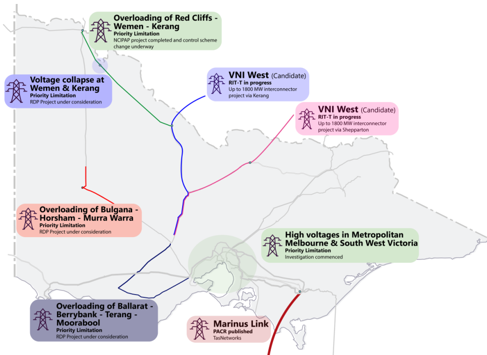
Figure 4 Transmission Development Plan for Victoria – future projects and priority limitations
