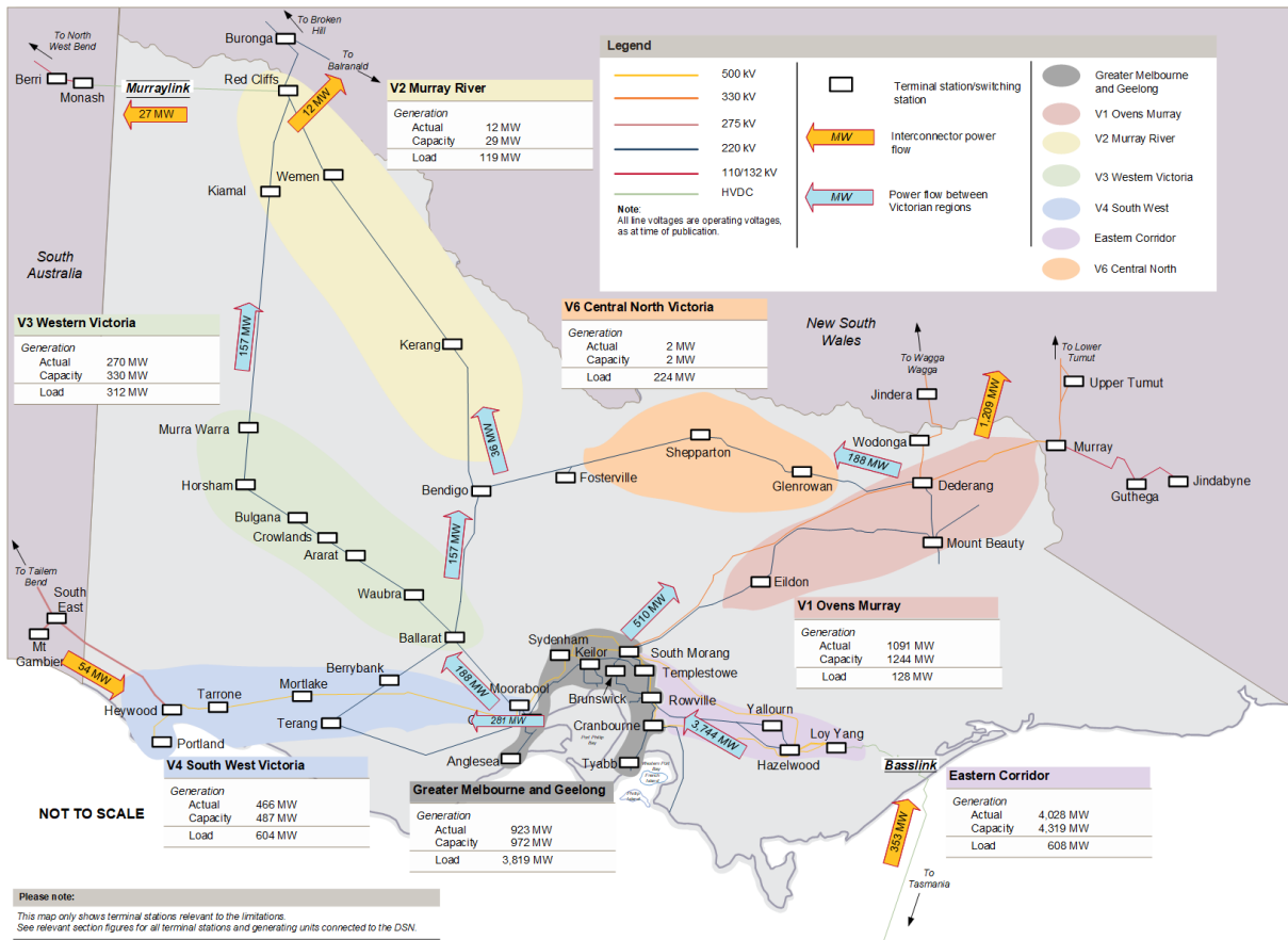
Figure 18 High export snapshot – generation, load, and interconnector flow
