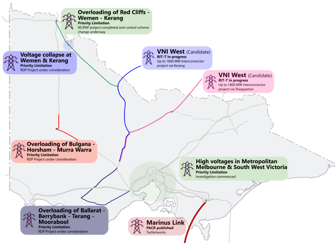
Figure 23 Transmission development plan – future projects and priority limitations
