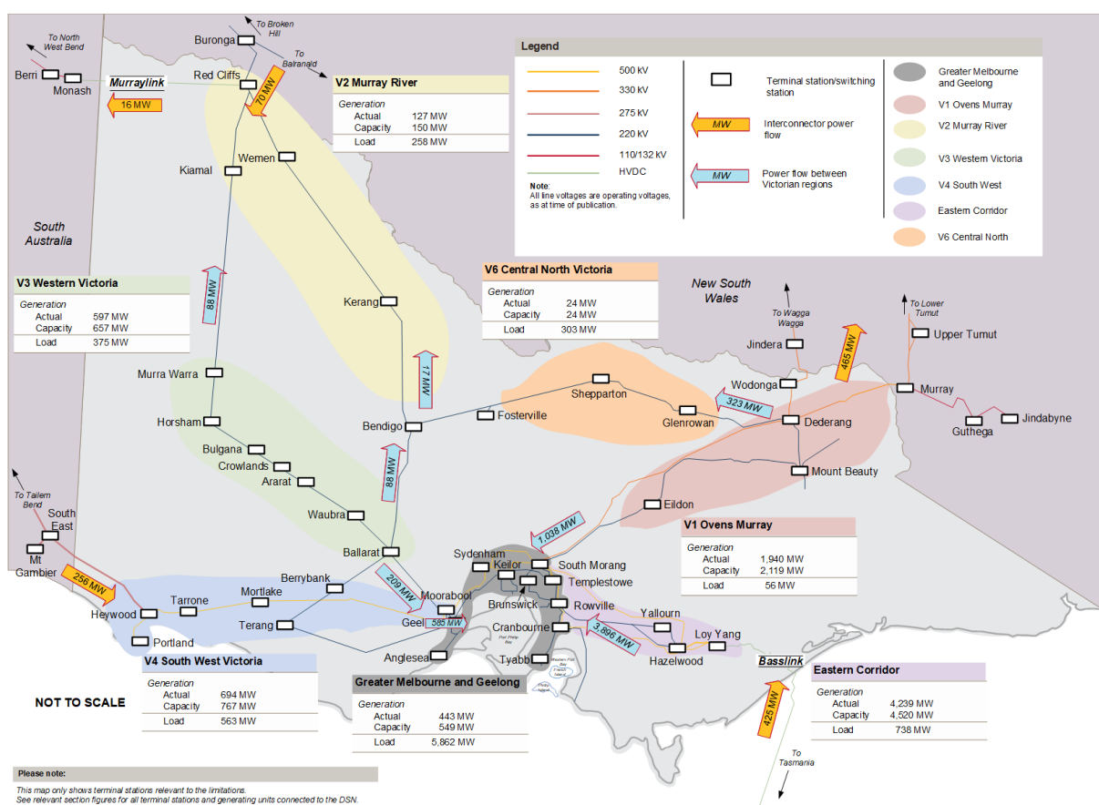
Figure 12 Maximum demand snapshot – generation, load, and interconnector flow
