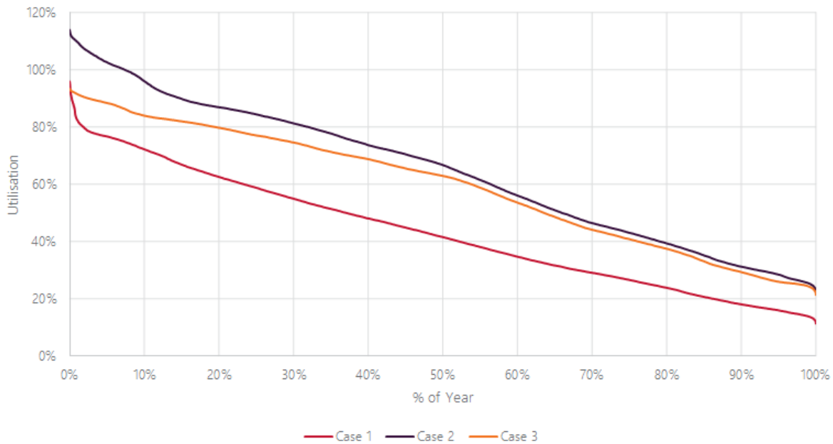
Figure 33 CBTS A1 500/220 kV transformer load duration curve
