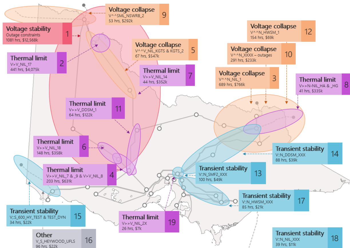
Figure 11 Map of the most significant Victorian transmission constraints in 2020-21
