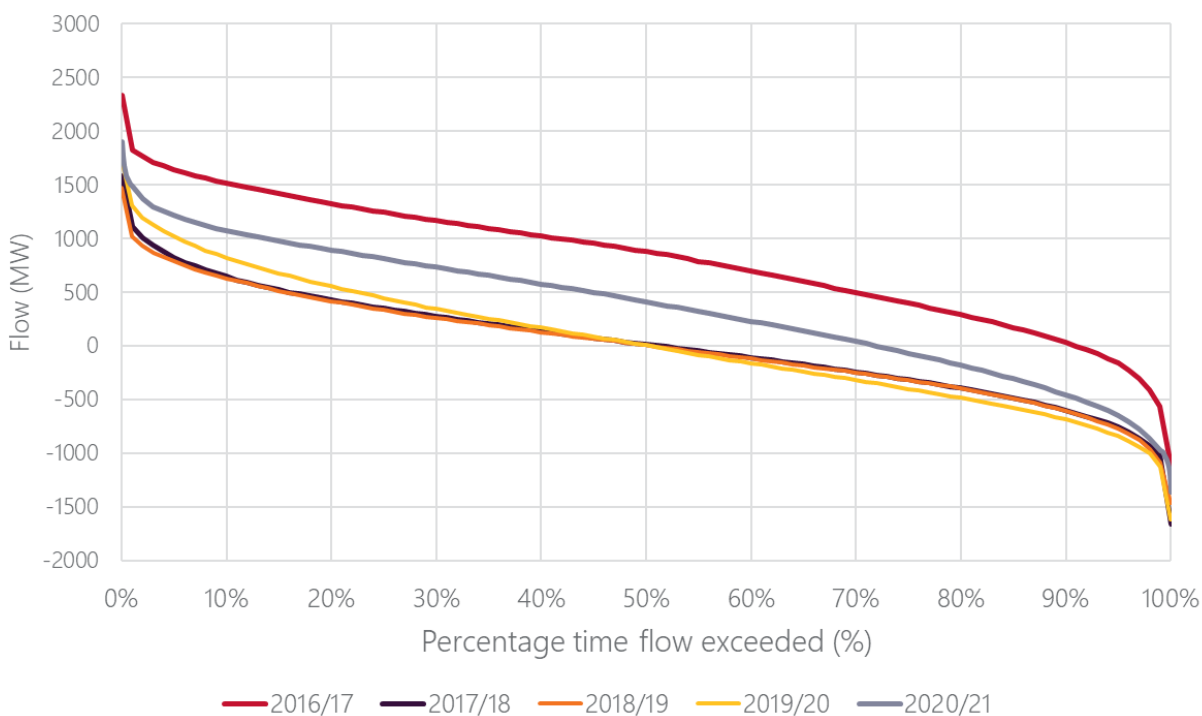
Figure 7 Victoria net export duration curve (all interconnectors)
