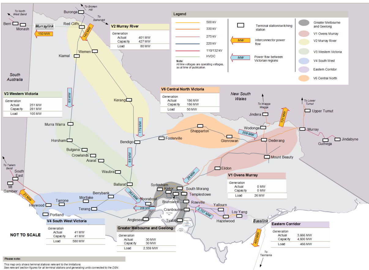
Figure 19 High solar snapshot – generation, load, and interconnector flow
