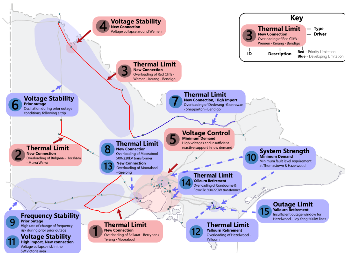
Figure 25 Priority limitations and developing limitations under investigation
