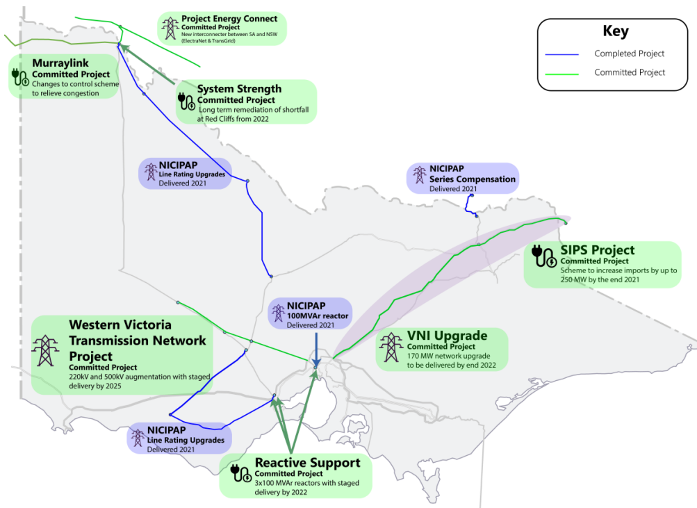
Figure 2 Transmission Development Plan for Victoria – delivered and committed projects
