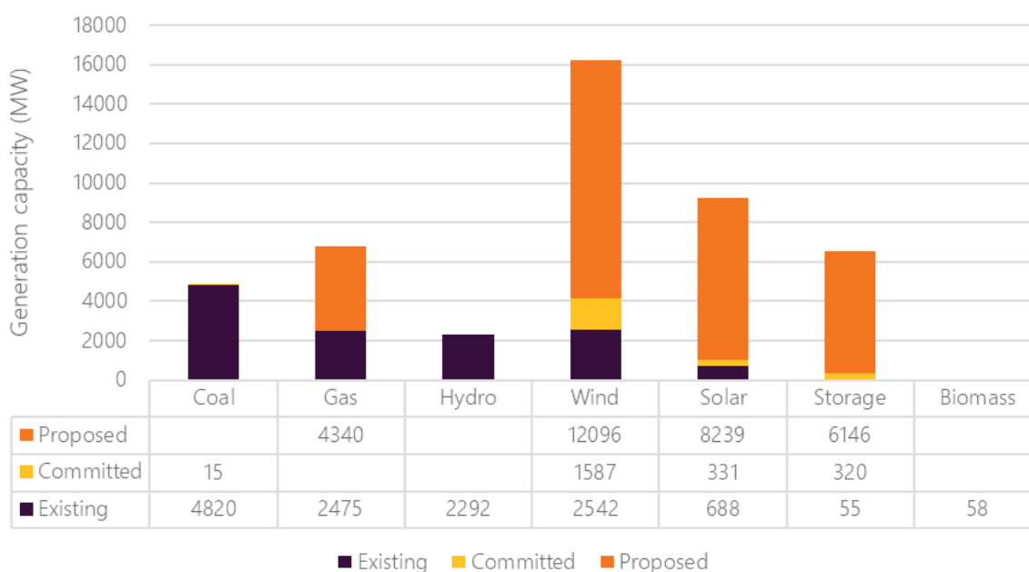
Figure 20 Existing, committed and proposed large-scale generation capacity in Victoria, October 2021
