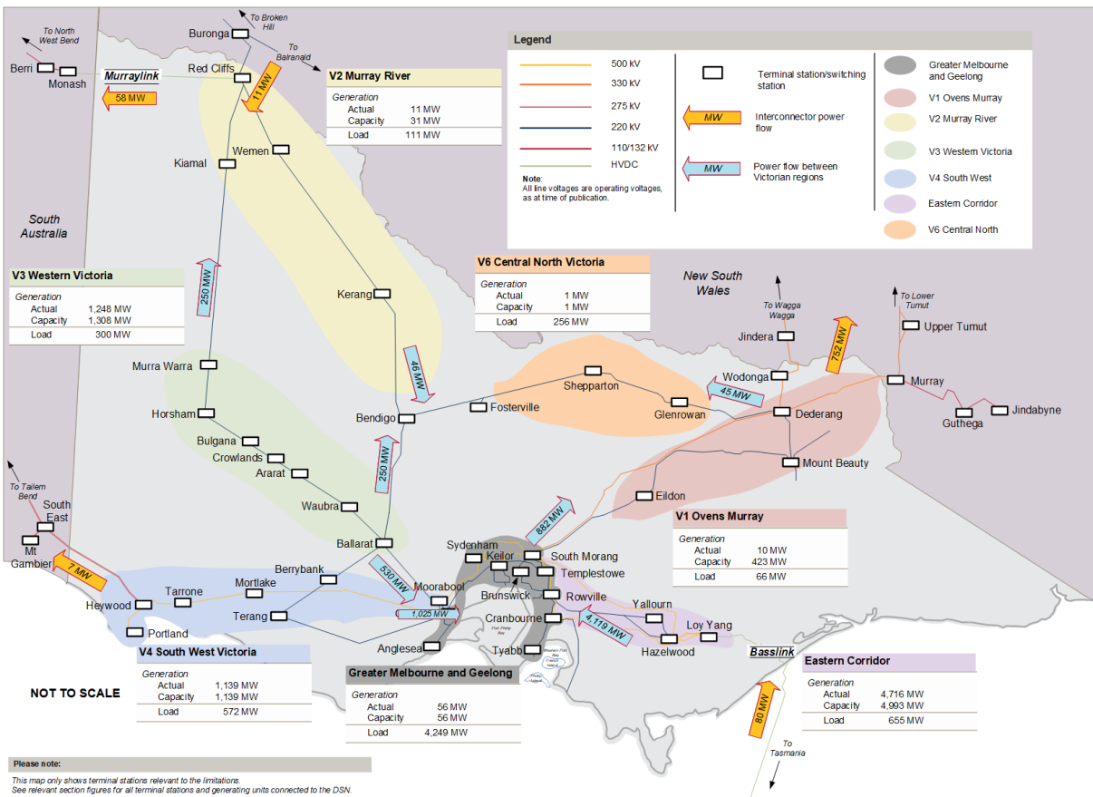
Figure 17 High wind snapshot – generation, load, and interconnector flow
