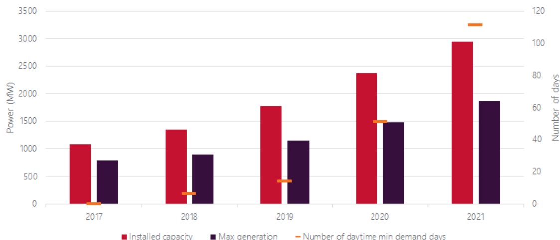
Figure 16 Rooftop PV capacity and maximum generation by financial year and number of daytime minimum demand days
