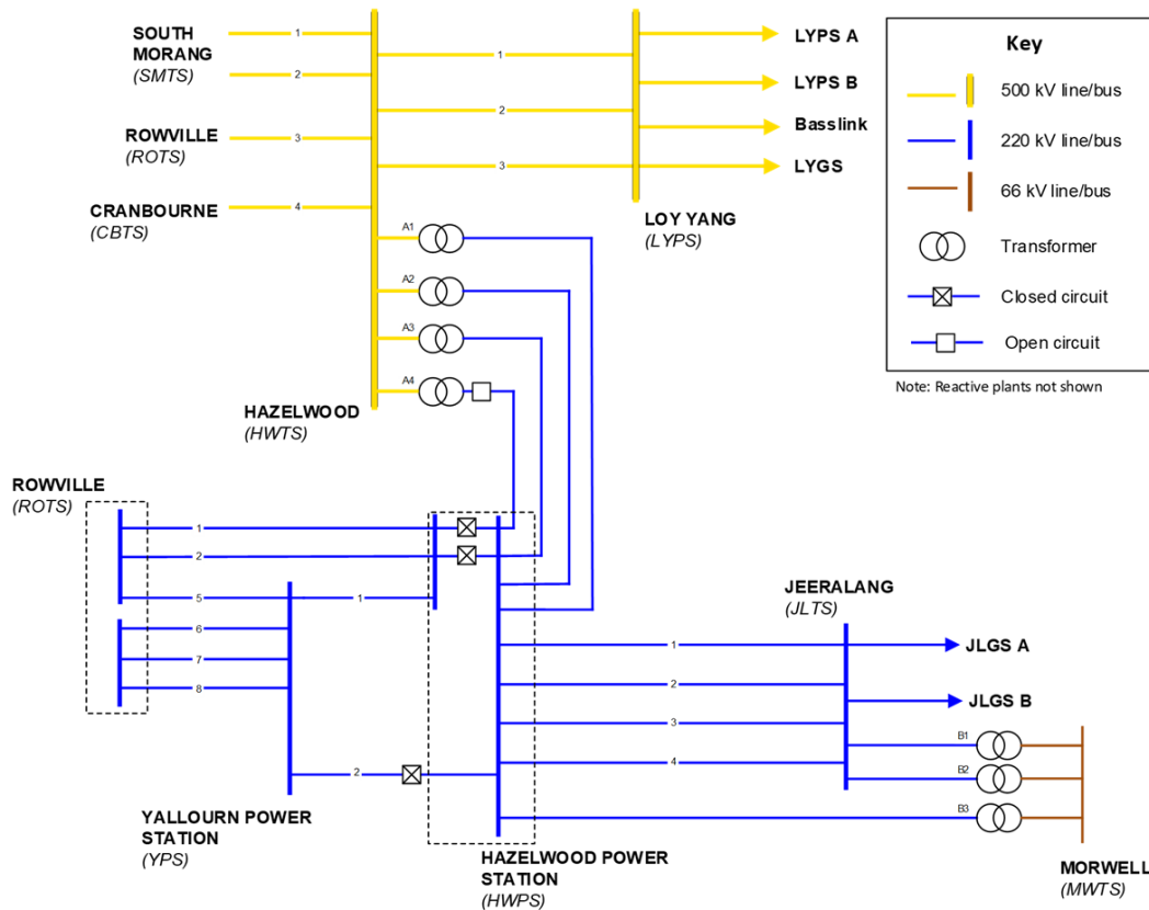
Figure 32 Latrobe Valley in parallel mode
