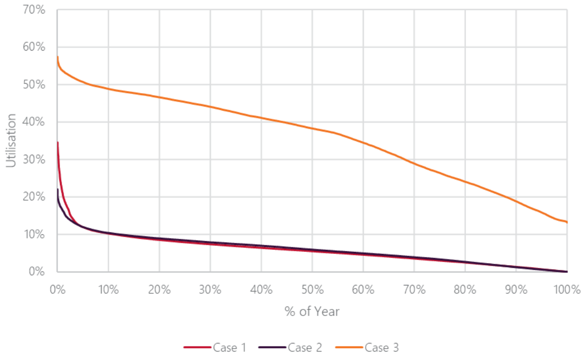
Figure 35 HWTS transformer load (under system normal) duration curve
