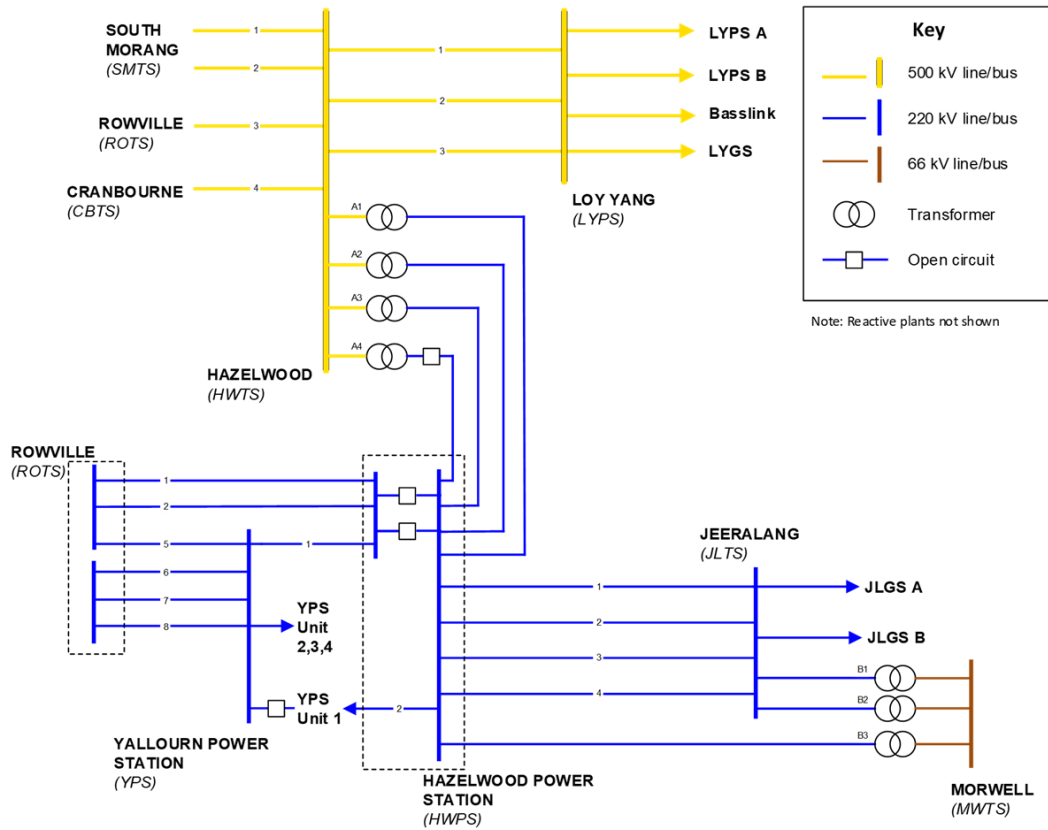
Figure 31 Latrobe Valley in radial mode
