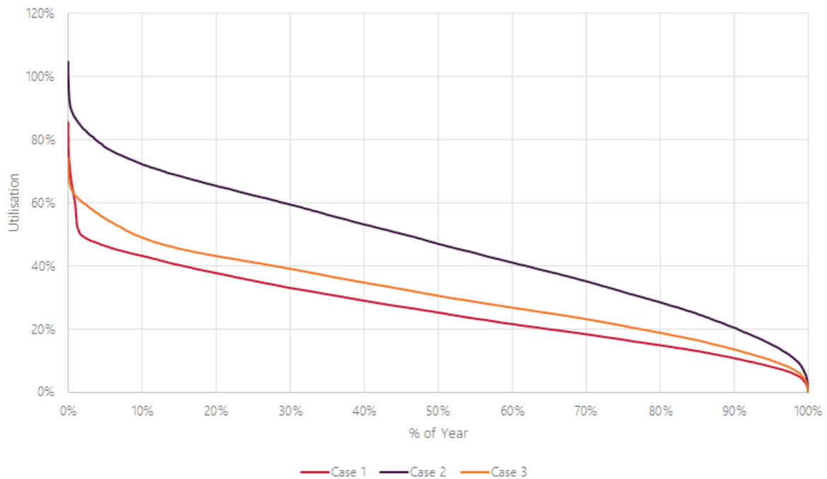
Figure 38 RWTS – TTS 220 kV line load (under contingency) duration curve
