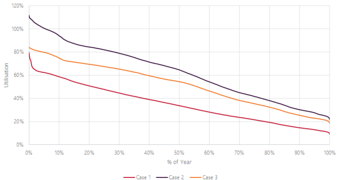
Figure 34 Rowville A1 500/220 kV transformer load duration curve
