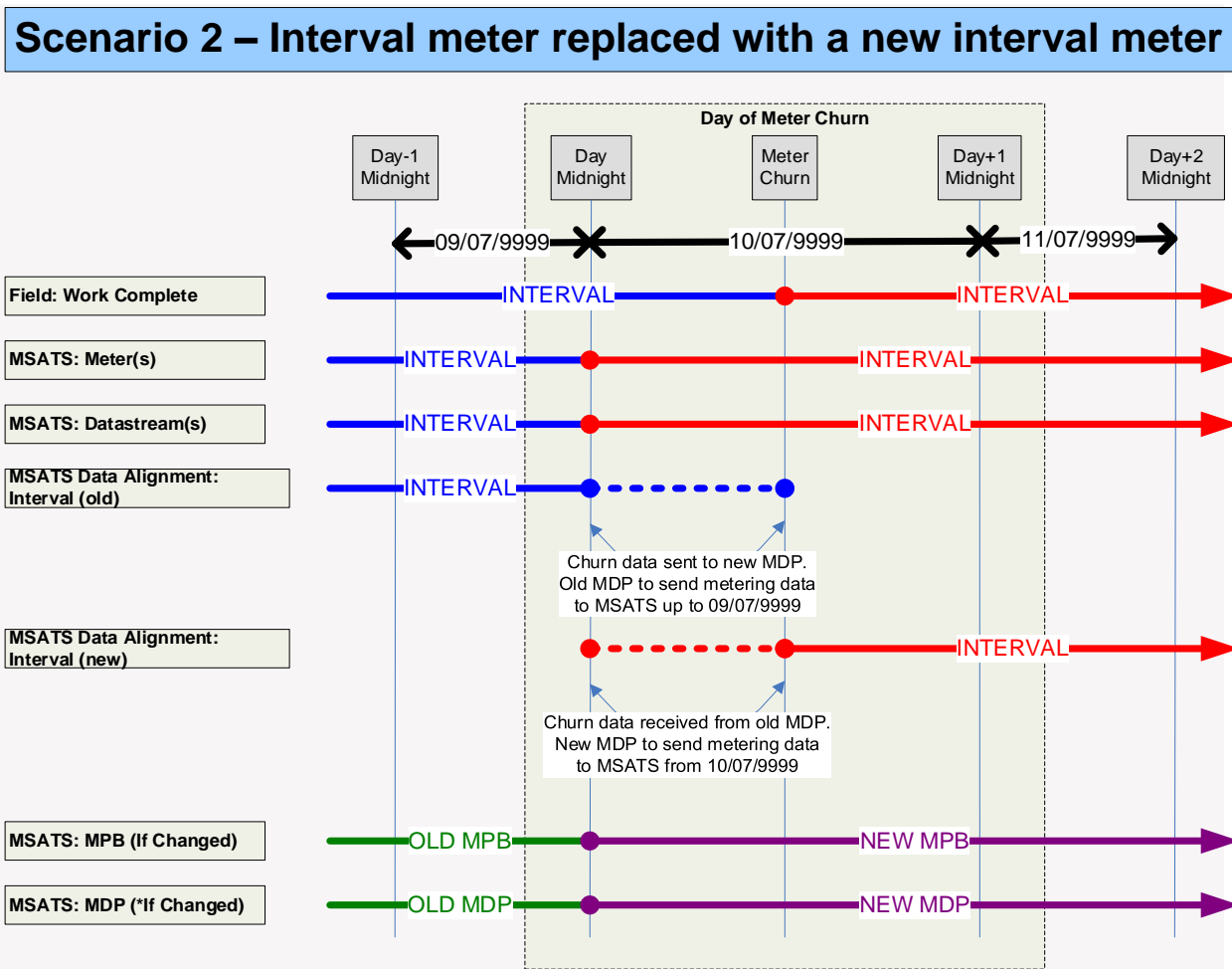
Figure 2 Scenario 2 – Interval Meter replaced with a new Interval Meter
