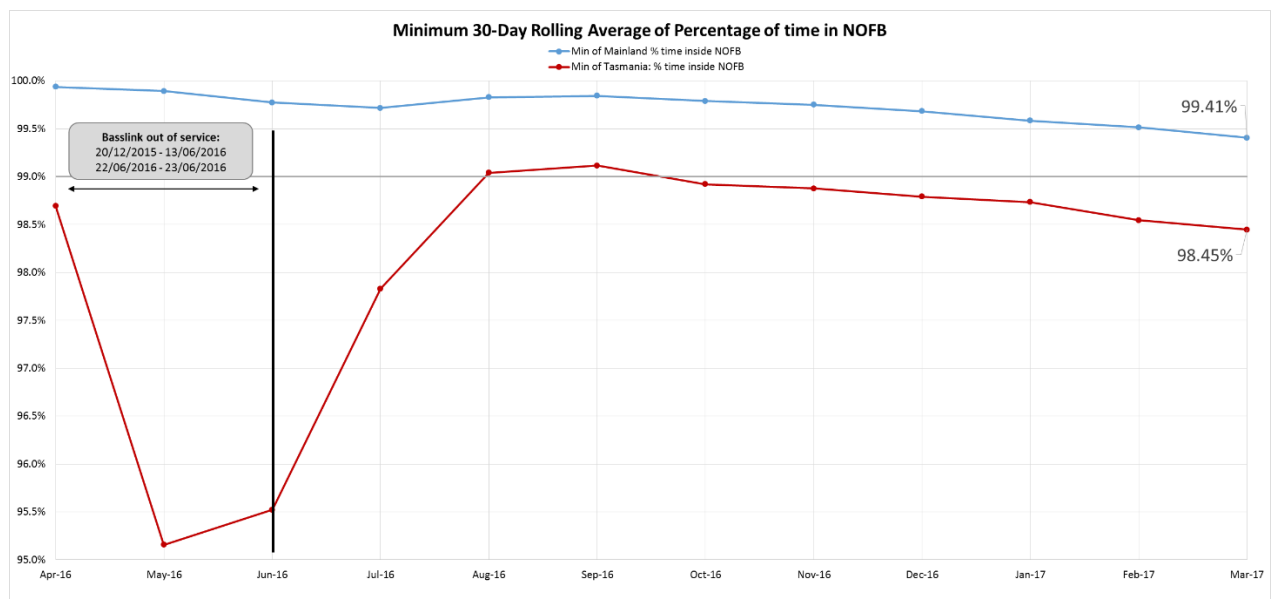
Figure 1 Minimum 30-Day rolling average of percentage of time mainland and Tasmania frequencies remained within NOFB from April 2016 to March 2017
