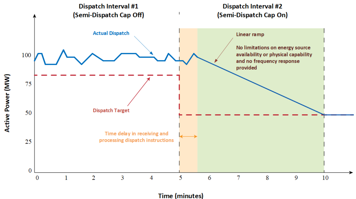
Figure 1 Semi-scheduled generating unit linear ramping with no limiting factors
