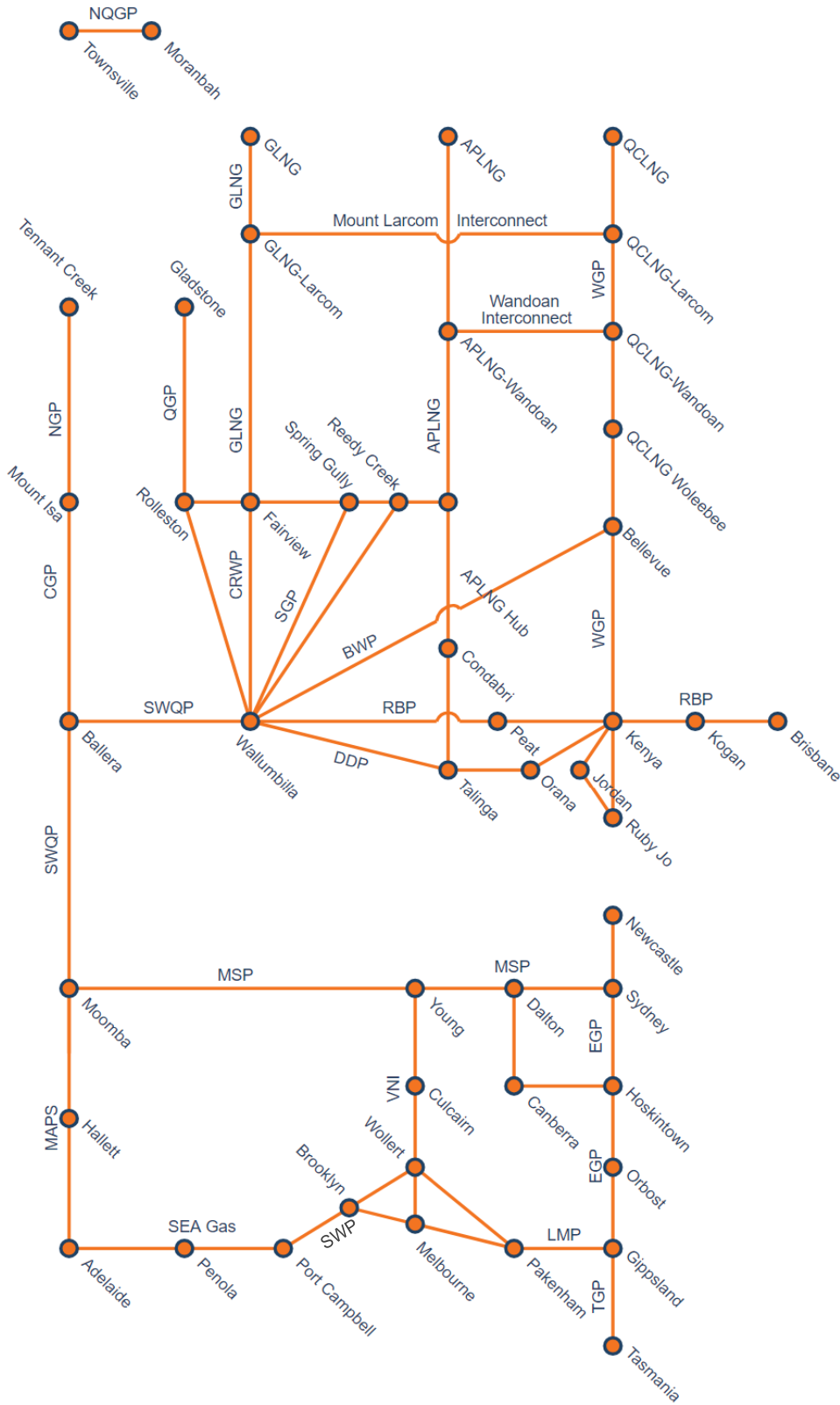
Figure 3 Gas model topology for 2022 GSOO
