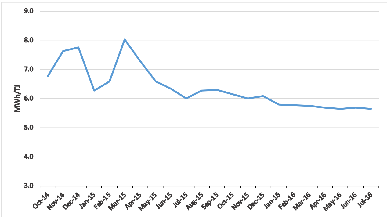
Figure 3-11 Electricity usage per unit of gas production, aggregate of fields in production (MWh/TJ)
