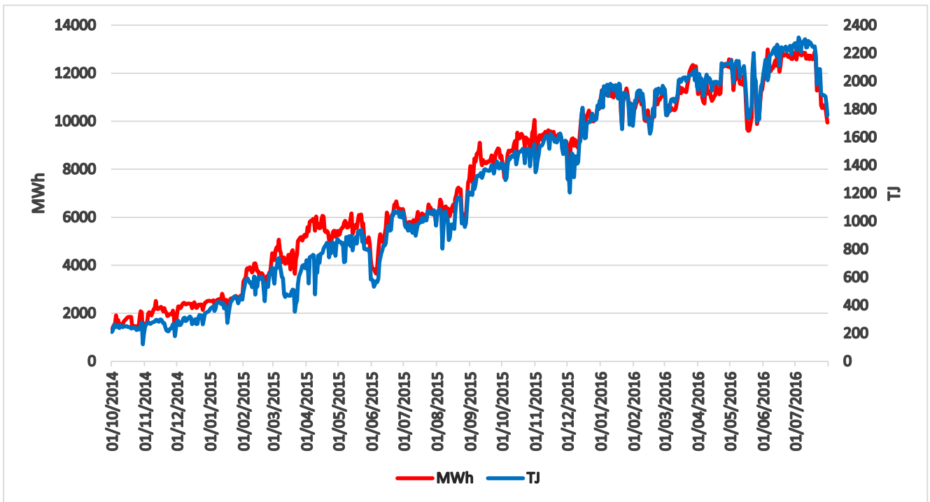
Figure 3-6 Aggregate daily electricity usage vs aggregate electricity powered gas production
