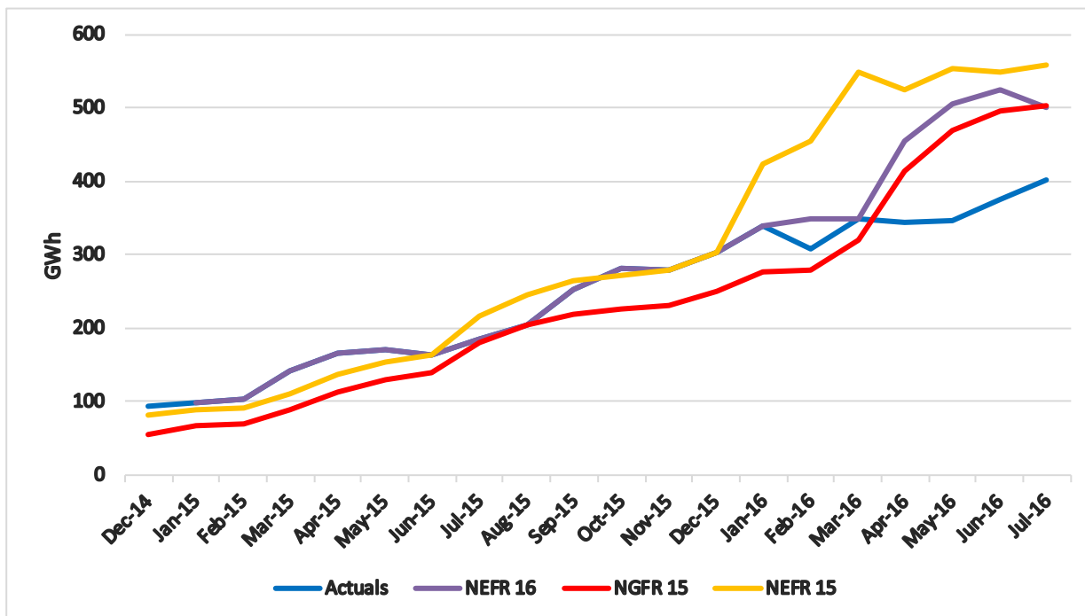
Figure 3-7 Projected vs Actual Electricity Usage (GWh)
