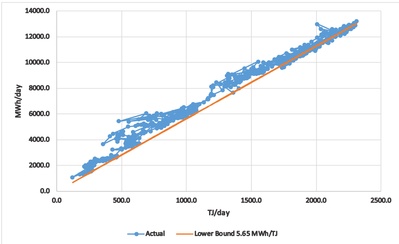
Figure 3-12 Aggregate daily electricity usage vs gas production
