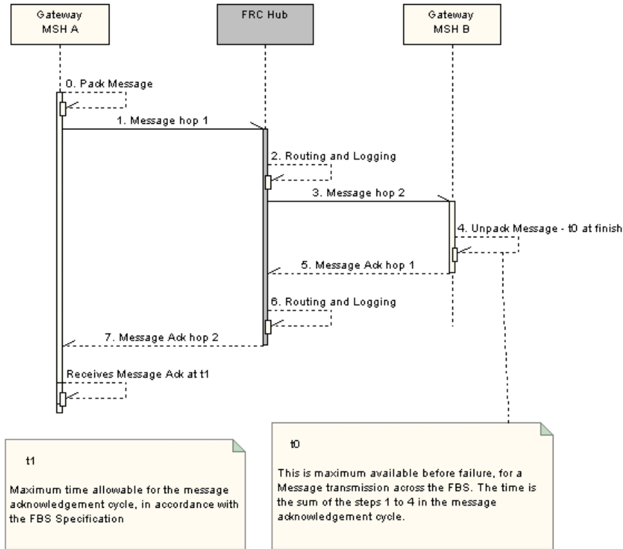
Figure 7 Timing steps in the Message cycle
