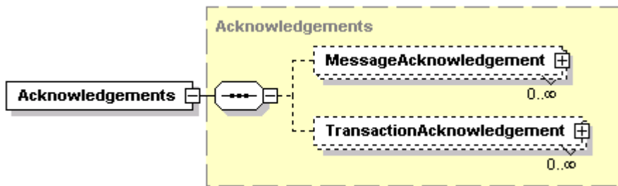
Figure 13 aseXML acknowledgments element format
