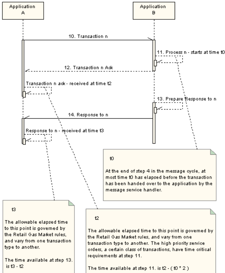
Figure 8 Timing steps in the transaction and response cycles
