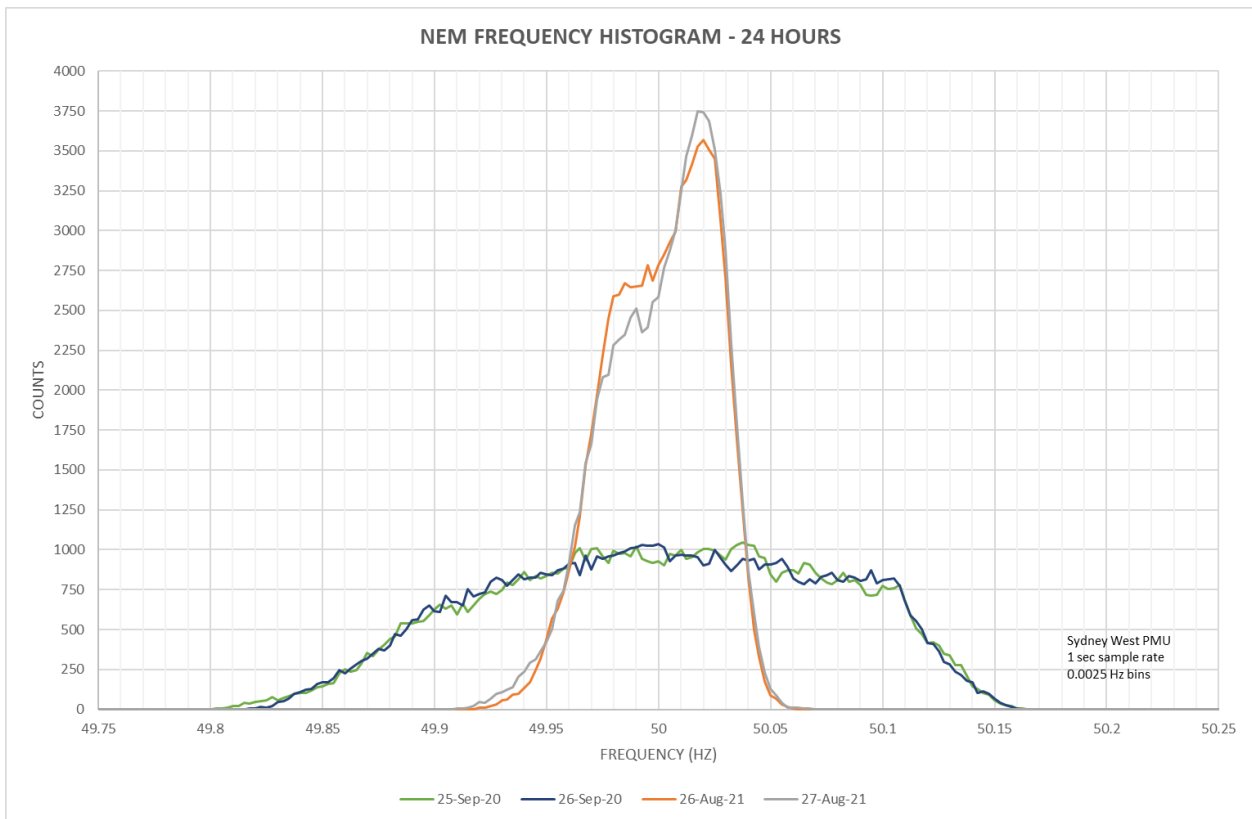
Figure 3 Comparison of NEM frequency distribution – Sep 2020 vs August 2021
