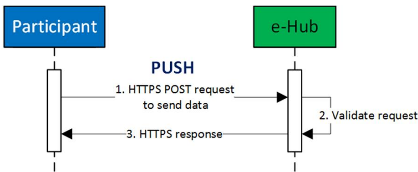
Figure 1 PUSH mechanism
