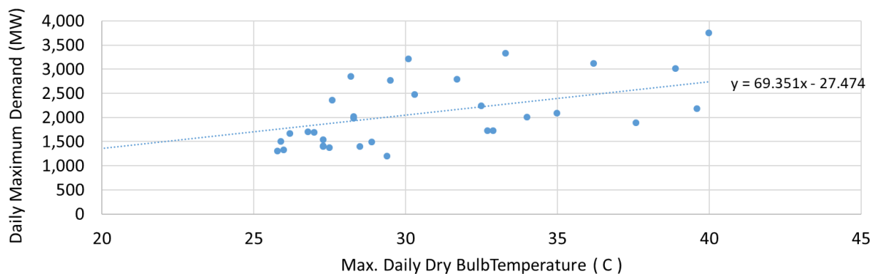
Figure 5 Figure 1 Estimated maximum daily residential demand vs maximum daily temperature, New South Wales
