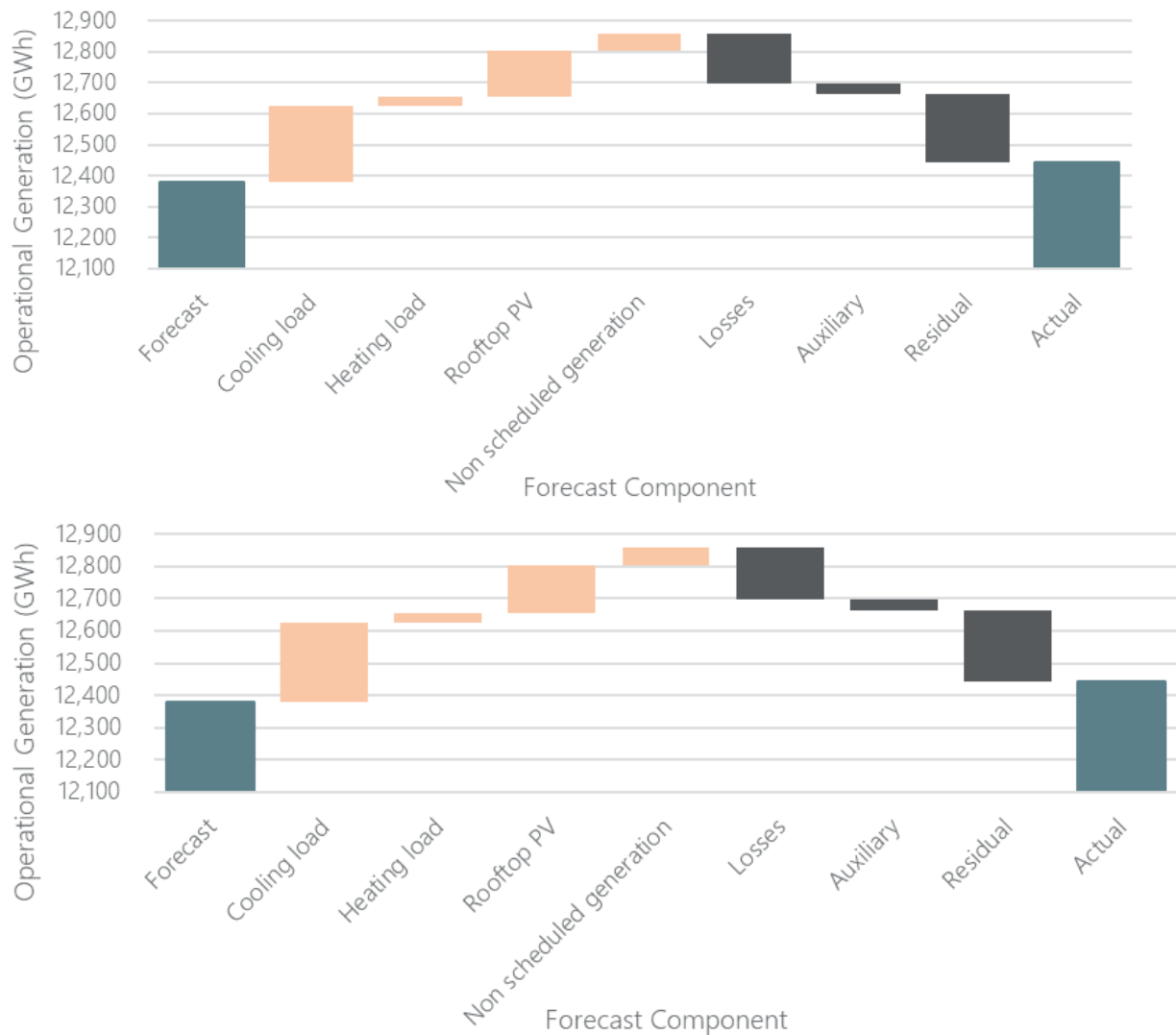
Figure 7 Example: Energy consumption component variance chart, South Australia
