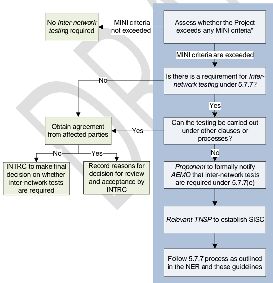
Figure 2 Assessment of whether inter-network test is required – activities 1 to 4 (see Appendix F)
