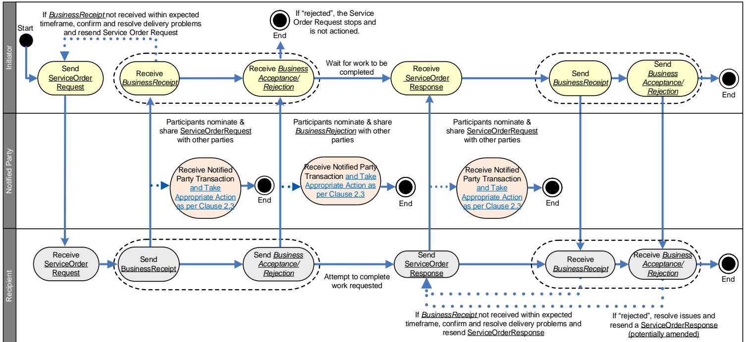
Figure 1 Service Orders
