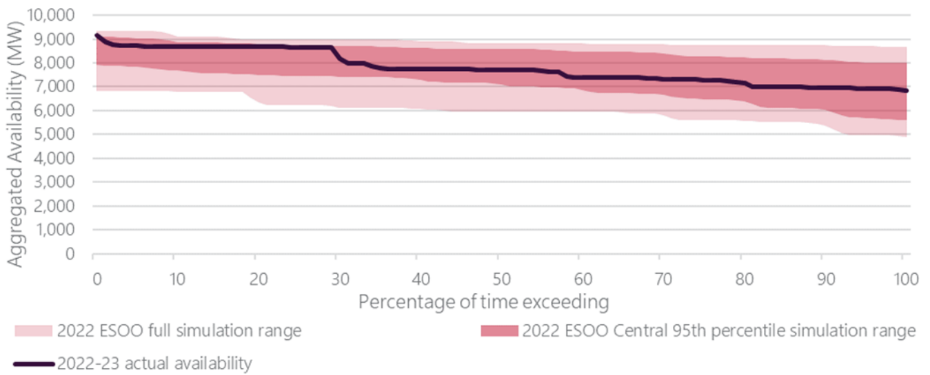
Figure 9 Example supply availability curve – New South Wales black coal, top 10 hottest days
