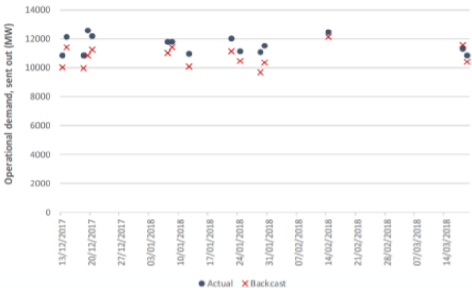
Figure 12 Actual versus backcast max demand half-hour for top 15 highest demand days in New South Wales
