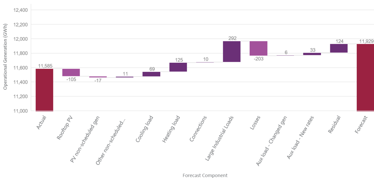
Figure 7 Example: Energy consumption component variance chart, South Australia
