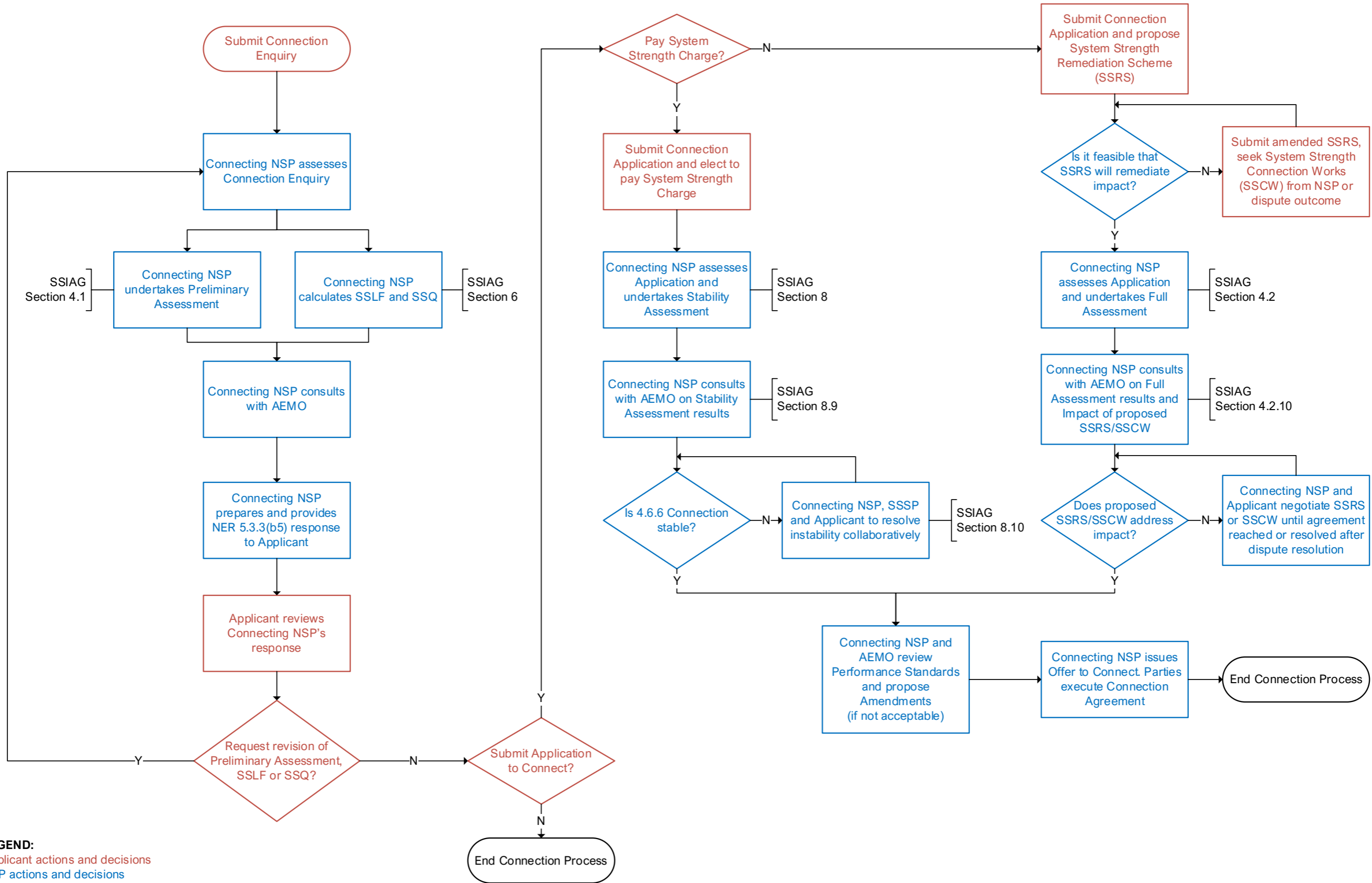
Figure 3 System strength impact assessment process within connection process
